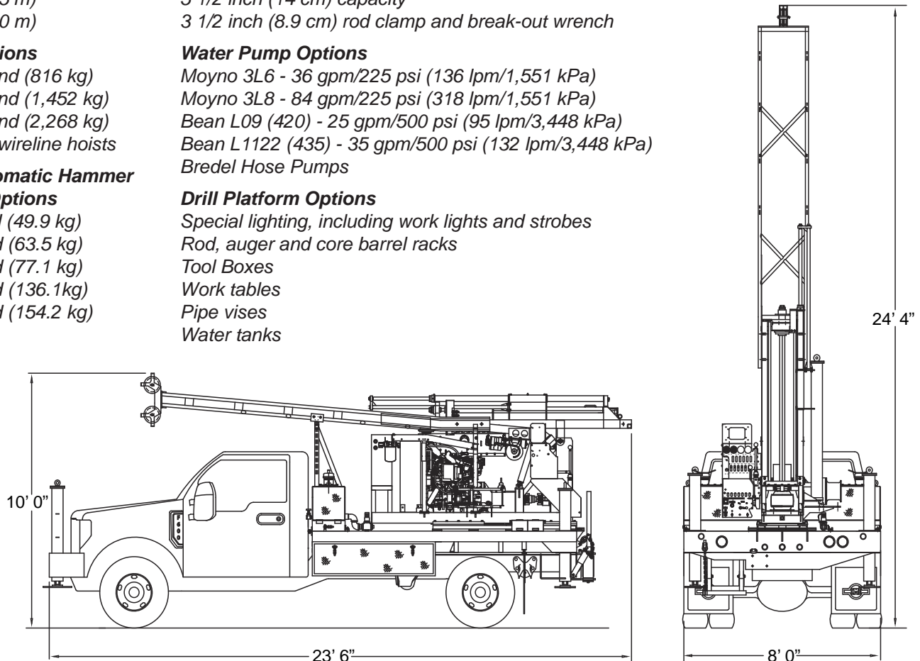
Typical truck mount configuration with optional 20 foot mast. Dimensions will vary, depending on truck wheelbase and options.
